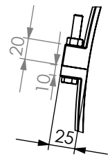
DETAIL A SCALE 1 : 5
